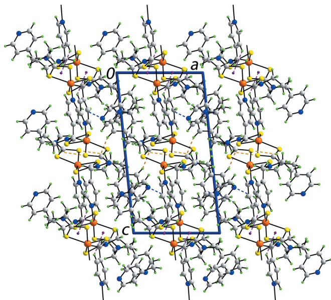
Figure 4 A view of the unit-cell contents in projection down the b axis. The C–H...S, C–H...N and C–H... \pi interactions are shown in orange, blue and purple dashed lines, respectively.
