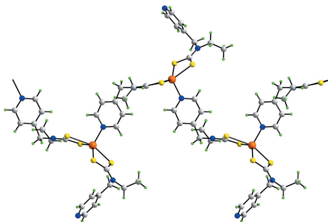
Figure 3 The one-dimensional coordination polymer in (I), aligned along [010].
