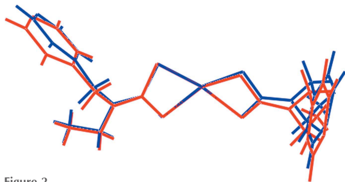
Figure 2 A molecular overlay diagram of the two independent molecules of \text{Zn}[\text{S}_2\text{CN}(\text{Et})\text{CH}_2\text{py}]_2 . The Zn1-containing molecule is shown in red and the molecules have been overlapped so that the two more symmetrically chelating dithiocarbamate ligands are coincident.
