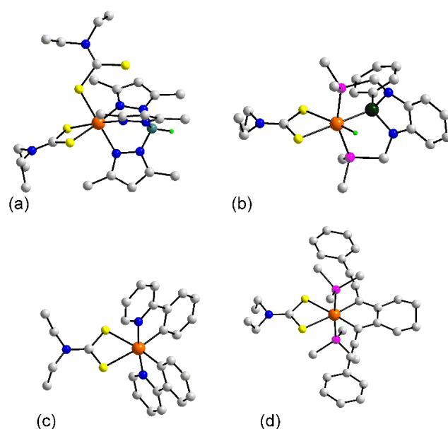
Figure 7. Molecular structures of rhodium complexes: (a) Tp*Rh( \eta^2 -L 24 )( \eta^1 -L 24 ) (73), (b) [Rh(H){ \kappa^3 -P,Si,P'-SiPh(NCH 2 PPh 2 ) 2 C 6 H 4 }(L 24 )] in the crystal of 74, (c) Rh(phpy) 2 (L 24 ) (75), and (d) (PMe 3 ) 2 Rh(X 2 )(L 24 ) (77). In (b), only the ipso-C atoms of the phosphane bound phenyl rings are shown for clarity.
