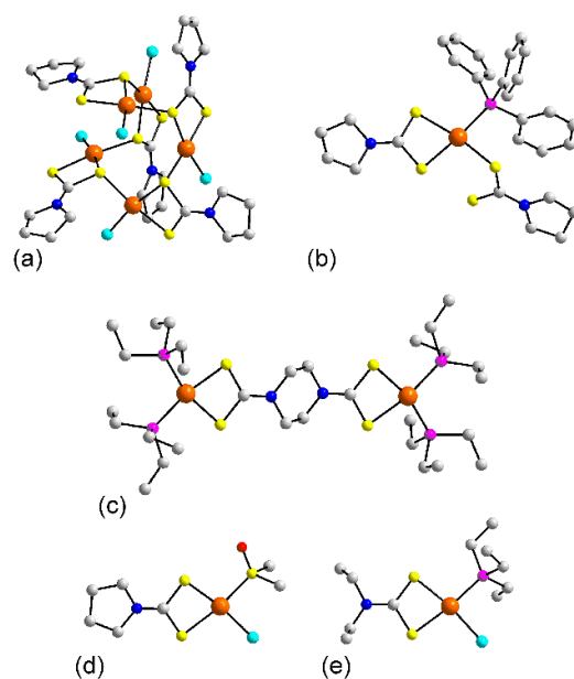
Figure 13. Molecular structures of platinum dithiocarbamate complexes: (a) [\text{Pt}(\text{L}^{57})\text{Cl}]_5 in the crystal of 233 , (b) (\text{PPh}_3)\text{Pt}(\eta^1\text{-L}^{57})(\eta^2\text{-L}^{57}) in 234 , (c) [(\text{PEt}_3)_2\text{Pt}]_2(\text{L}^{74})^{2+} in 235 , (d) \text{Pt}(\text{L}^{57})\text{Cl}((\text{CH}_3)_2\text{SO}) ( 237 ), and (e) (\text{PEt}_3)\text{Pt}(\text{L}^{24})\text{Cl} ( 238 ).
