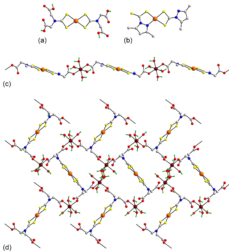
Figure 12. Molecular structures of platinum dithiocarbamate complexes: (a) \text{Pt}(\text{L}^{52})_2 ( 222 ) and (b) \text{Pt}(\text{L}^{62})_2 ( 228 ), and coordination polymers in (c) [\text{Zn}(\text{H}_2\text{O})_4\text{Pt}(\text{L}^{17})_2]_n in the crystal of 229 and (d) [[\text{Zn}(\text{H}_2\text{O})_4]_2\text{Pt}(\text{L}^{51})_2]_n in 232 .
