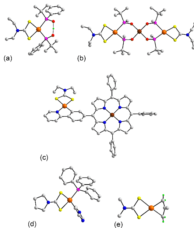
Figure 9. Molecular structures of palladium complexes: (a) [tBu(Ph)POH][tBu(Ph)P(=O)]Pd(L 24 ) ( 147 ), (b) Cu{[tBu(PhP)(O)]Pd(L 24 )} 2 ( 148 ), (c) Pd(X 3 )(L 24 ) in 152 , (d) (PPh 3 )Pd(pyr)(L 57 ) ( 154 ), and (e) Pd(η 3 -C 4 H 7 )(L 8 ) ( 155 ). In (b), only the ispo-C atoms of the phosphane bound phenyl rings are shown for clarity.
