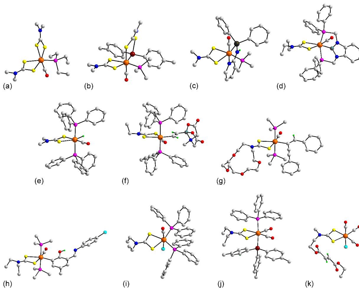
Figure 4. Molecular structures of ruthenium complexes: (a) (PEt_3)Ru(L^8)_2(CO) ( 22 ), (b) (PPh_3)Ru\{Ge(p\text{-tolyl})_2\}(L^8)_2(CO) in the crystal of 23 , (c) (PPh_3)Ru(\kappa^2(Si,N)\text{-}SiPh_2NHC_5H_4N)(L^8)(CO) ( 24 ), (d) Ru(B(NCH_2PPh_2)_2C_6H_4)(L^{24})(CO) ( 27 ), (e) (PPh_3)_2Ru(H)(L^8)(CO) ( 29 ), (f) (PPh_3)_2Ru(C(H)=C(H)BMIDA)(L^{24})(CO) in 33 , (g) (PPh_3)_2Ru(C(C\equiv C(Ph)=C(H)Ph)(L^{84})(CO) ( 38 ), (h) (PPh_3)_2Ru(X)(L^{24})(CO) ( 43 ), (i) (PPh_3)_2Ru(L^{24})(CO)Cl in 44 , (j) (PPh_3)Ru(Ge(p\text{-tolyl})_3)(L^{24})(CO)_2 ( 48 ), and (k) Ru(L^{22})(CO)_3Cl ( 49 ). In (b,c,g,h), only the ipso-C atoms of the phosphane bound phenyl rings are shown for clarity. Additional color code: silicon, dark green; boron, teal.
