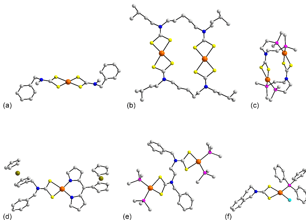
Figure 8. Molecular structures of palladium complexes: (a) \text{Pd}(\text{L}^{13})_2 ( 81 ), (b) \text{Pd}(\text{L}^{86})_2 in the crystal of 100 , (c) [\text{Pd}_2(\text{L}^{44})_2]^{2+} in 102 , (d) (\text{fcdpm})\text{Pd}(\text{L}^{43}) ( 105 ), (e) \{[(\text{PPh}_3)_2\text{Pd}]_2(\text{L}^{85})\}^{2+} in 113 , and (f) (\text{PPh}_3)\text{Pd}(\text{L}^{81})\text{Cl} in 122 . In (c,e), only the ipso-C atoms of the phosphane bound phenyl rings are shown for clarity.
