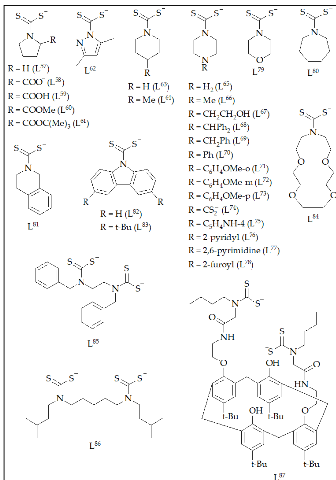
Figure 2. Chemical diagrams of dithiocarbamates L 57 to L 87 .
