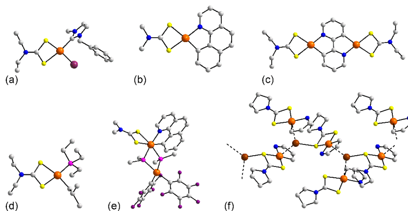
Figure 14. Molecular structures of platinum dithiocarbamate complexes: (a) Pt(bmi)(L 24 )I ( 244 ), (b) Pt(bzq)(L 8 ) ( 245 ), (c) [Pt(L 24 )] 2 (bpy) in the crystal of 248 , (d) (PEt 3 )Pt(L 24 )(CH 2 (iPr)) ( 249 ), (e) Pt(bzq)(L 8 )(PPh 2 ) 2 Pt(C 6 F 5 ) 2 ( 251 ), and (f) the coordination polymer [Ag{Pt(bzq)(L 57 )}] n in 252 . In (f), only the atoms forming the chelate ring formed by the benzo[h]quinolin-10-yl ligand are shown.
