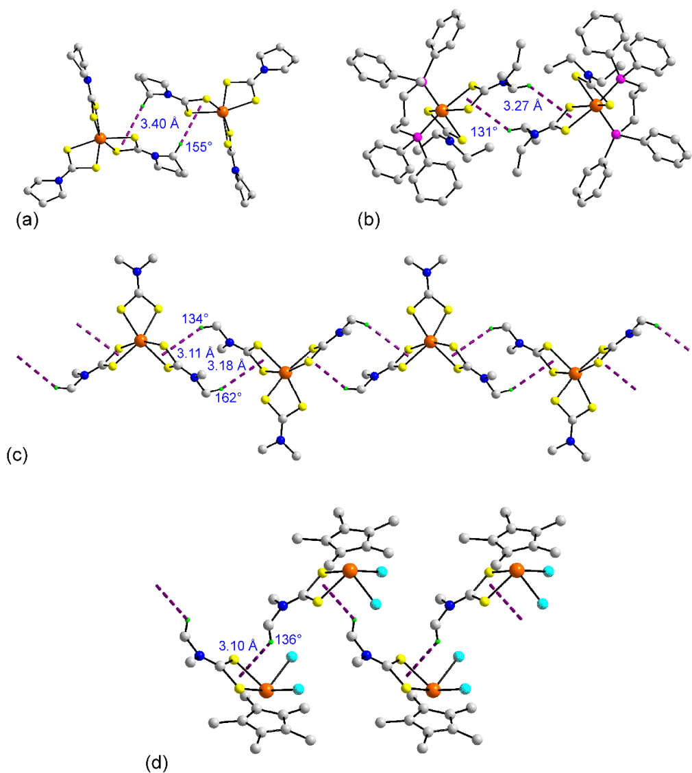
Figure 6. Supramolecular aggregation between molecules in the crystals of (a) 3 , (b) 8 , (c) 1 , and (d) 58 . The C–H... \pi (RuS 2 C) interactions are represented by dashed purple lines, and the distances and angles associated with the C–H... \pi (RuS 2 C) interactions are given on each image.
