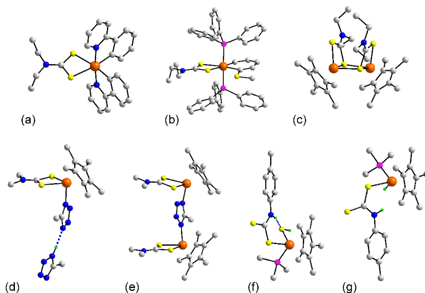
Figure 11. Molecular structures of iridium dithiocarbamate complexes: (a) \text{Ir}(\text{ppy})_2(\text{L}^{24}) (177), (b) (\text{PPh}_3)_2\text{Ir}(\text{C}_5\text{H}_5\text{SMe})(\text{L}^{24}) (199), (c) [\text{Cp}^*\text{Ir}(\text{L}^{24})]^{2+} in the crystal of 204, (d) \text{Cp}^*\text{Ir}(\text{mtz})(\text{L}^8) in 205, (e) [\{\text{Cp}^*\text{Ir}(\text{L}^8)\}_2(\text{mtz})]^+ in 206, (f) \text{Cp}^*\text{Ir}(\text{PMe}_3)(\text{L}^5)(\text{SH}) in 207, and (g) \text{Cp}^*\text{Ir}(\text{H})(\text{PMe}_3)(\text{L}^5) (208). In (d) and (f), the blue dashed line represents \text{N}-\text{H}\cdots\text{N} and \text{N}-\text{H}\cdots\text{S} hydrogen bonds, respectively.
