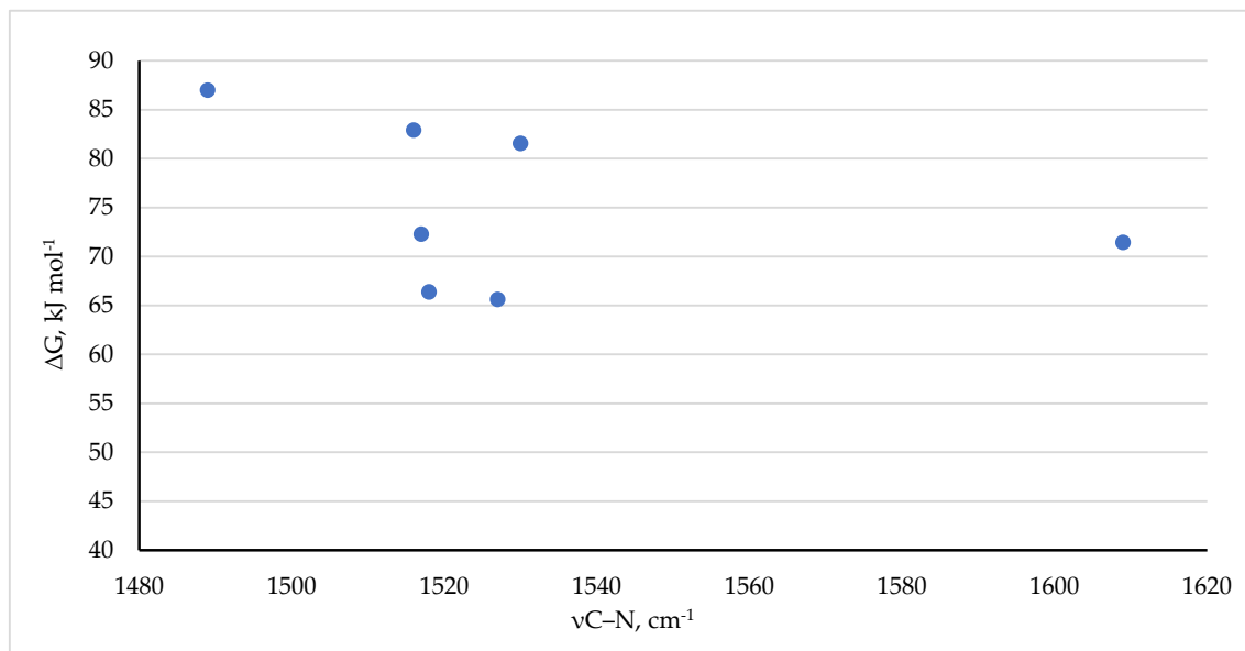
Figure 17. Correlation of \nu_{\text{C-N}} with the barrier to C–N bond rotation.
