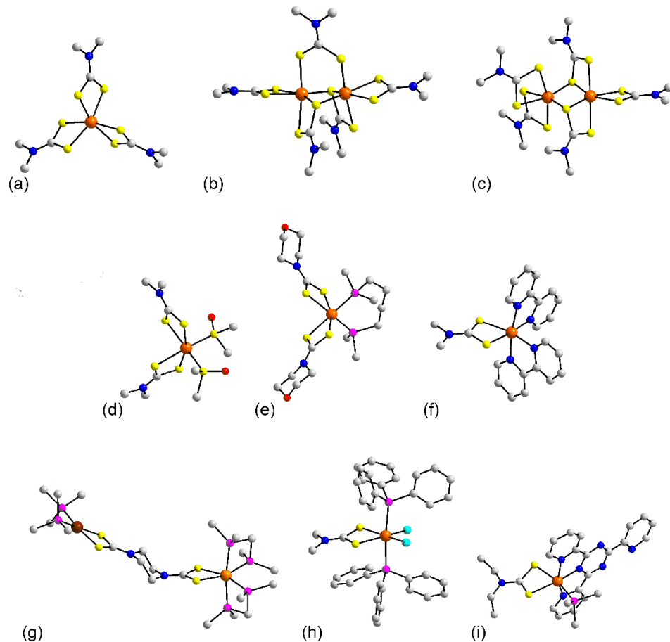
Figure 3. Molecular structures of ruthenium complexes: (a) Ru(L^8)_3 ( 1 ), (b) [Ru(L^8)_3] in the crystal of 4 , (c) [Ru_2(L^8)_3] in 5 , (d) Ru(L^8)_2((CH_3)_2SO)_2 ( 6 ), (e) (dppb)Ru(L^7)_2 ( 10 ), (f) [Ru(bpy)_2(L^8)]^+ in 11 , (g) [(dppm)_2Ru(L^7)_4Pd(PPh_3)_2]^{2+} in 17 , (h) [(PPh_3)_2Ru(L^8)Cl_2] in 18 , and (i) [(PPh_3)Ru(tptz)(L^{24})]^+ in 21 . In (e,g,i), only the ipso-C atoms of the phosphane bound phenyl rings are shown for clarity. Color code in this and subsequent crystallographic images: platinum-group element, orange; other heavy element, brown; chloride, cyan; sulfur, yellow; phosphorus, purple; oxygen, red; nitrogen, blue; carbon, grey; hydrogen, green. Non-participating H atoms are omitted.
