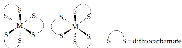
Figure 16. L- and D-forms of [M(L-L) 3 ].
