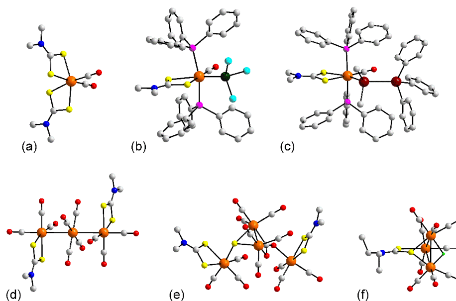
Figure 10. Molecular structures of osmium complexes: (a) Os(L 8 ) 2 (CO) 2 ( 157 ), (b) (PPh 3 ) 2 Os(SiCl 3 )(L 8 )(CO) in the crystal of 158 , (c) (PPh 3 ) 2 Os(SnMe 2 SnPh 3 )(L 8 )(CO) in 170 , (d) Os 3 (L 8 ) 2 (CO) 10 ( 173 ), (e) Os 4 (L 8 ) 2 (CO) 12 (CO 2 )(S) in 174 , and (f) Os 3 (H)(L 24 )(CO) 9 ( 176 ).
