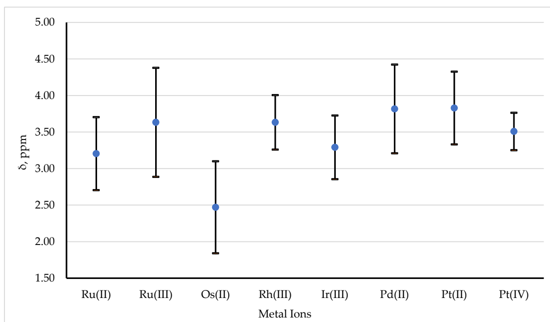
Figure 15. The mean and 95% range (two standard deviations) for the ^1\text{H} chemical shifts reported for \alpha -hydrogen nuclei.
