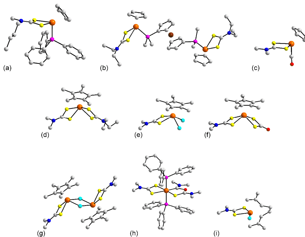
Figure 5. Molecular structures of ruthenium complexes: (a) \text{CpRu}(\text{PPh}_3)(\text{L}^{11}) ( 50 ), (b) \{[\text{CpRu}(\text{L}^{24})]_2(\text{dppf})\} in the crystal of 54 , (c) \text{CpRu}(\text{L}^8)(\text{CO}) ( 55 ), (d) [\text{Cp}^*\text{Ru}(\text{L}^8)(\text{L}^{24})]^+ in 57 , (e) \text{Cp}^*\text{Ru}(\text{L}^8)\text{Cl}_2 ( 58 ), (f) \text{Cp}^*\text{Ru}(\text{S}_2\text{C}=\text{O})(\text{L}^8) ( 60 ), (g) [\text{Cp}^*\text{Ru}(\text{L}^8)\text{Cl}]_2^{2+} in 64 , (h) [(\text{PPh}_3)_2\text{Ru}(\text{C}(\text{NMe}_2)\text{OC}(\text{NMe}_2)=\text{S})(\text{L}^8)]^+ in 67 , and (i) \text{Ru}(\text{X}^1)(\text{L}^8)\text{Cl} ( 69 ). In (b), only the ipso-C atoms of the phosphane bound phenyl rings are shown for clarity.
