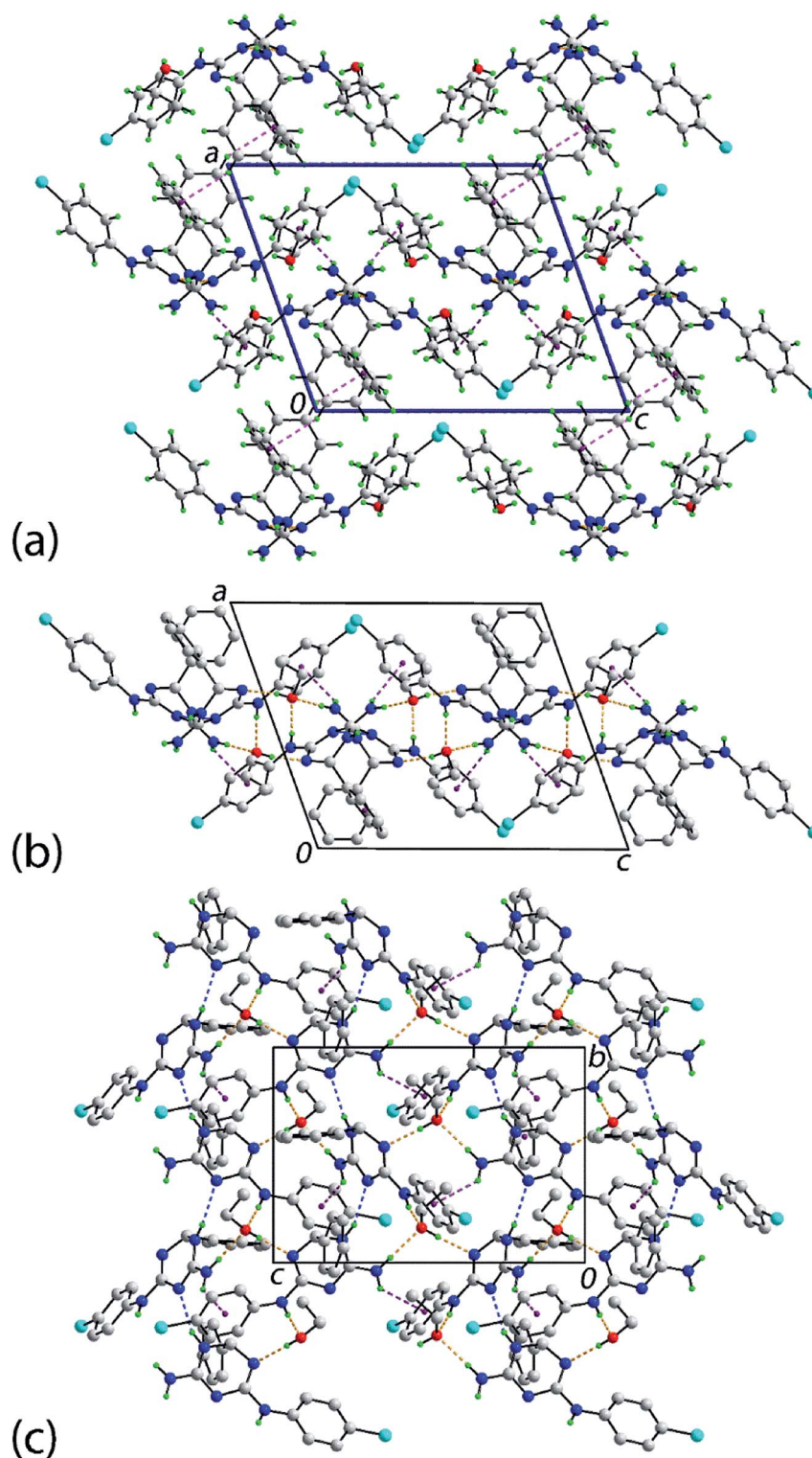
Fig. 2 Molecular packing in the crystal of 1e ·EtOH: (a) a view of the unit cell contents in projection down the b -axis. The N–H···N, N–H···π and C–H···π interactions are shown as blue, purple and pink dashed lines, respectively. (b) A side-on view of a supramolecular layer highlighting the encapsulation of the solvent ethanol molecules and (c) a plan view of the layer shown in (b). Hydrogen-bonding interactions involving ethanol are indicated by orange dashed lines. For (b) and (c), non-participating hydrogen atoms are omitted for reasons of clarity.
